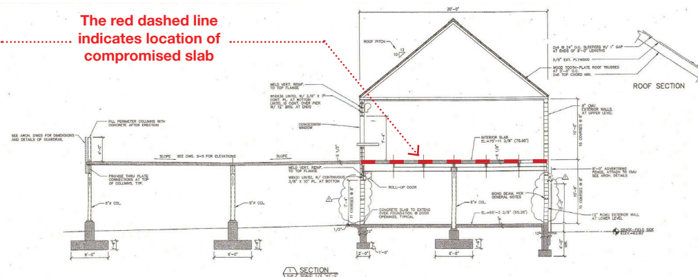
Fig 034. Outfield Building Section
