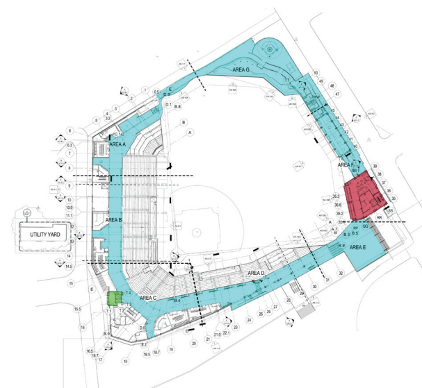
Fig. 215. Main Concourse Level Plan
