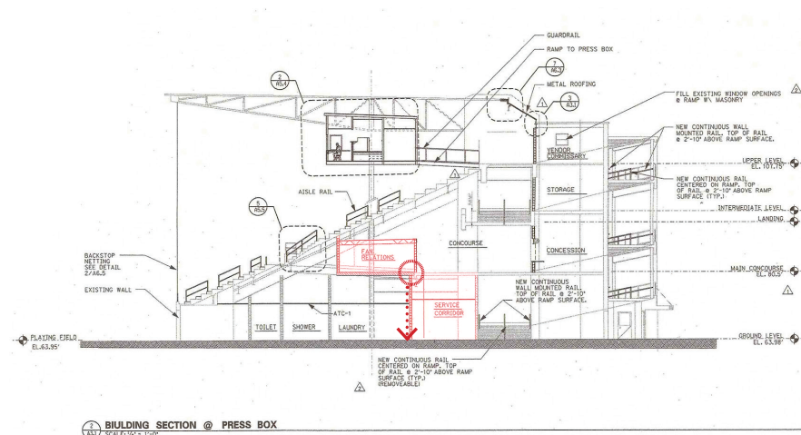
Fig 041. McCoy Building Section
