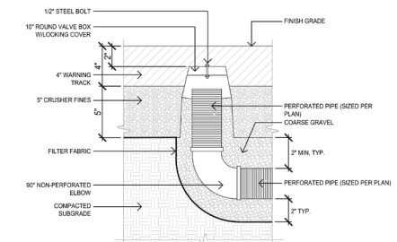
Fig. 092. Modern Playing Field Section
