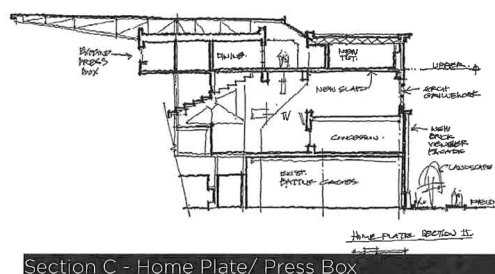
Fig. 009. Populous 2015 Report - Proposed Redevelopment Section
