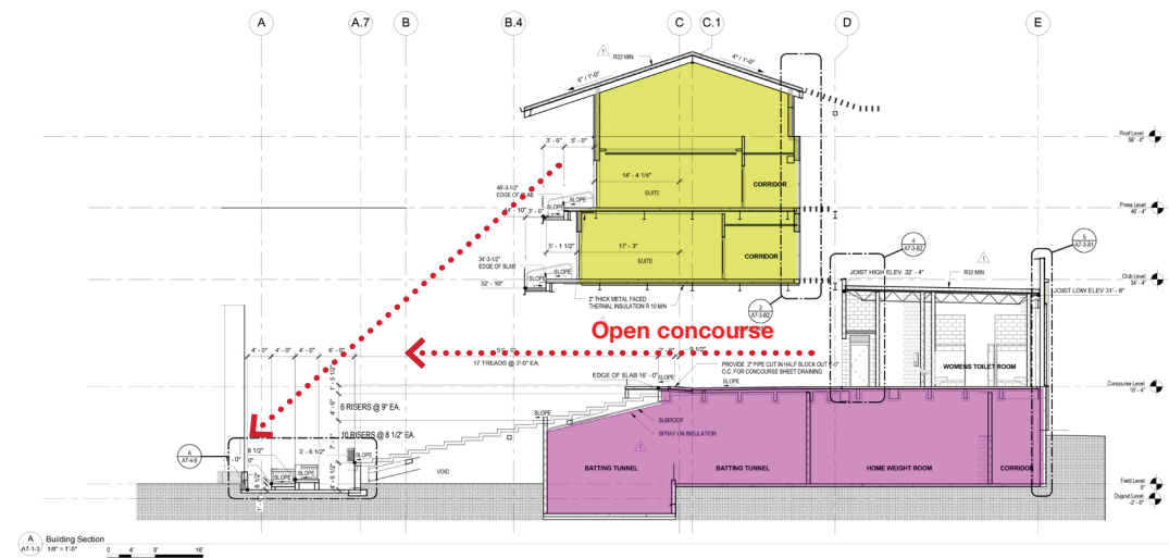
Fig. 217. Southwest University Park Building Section
