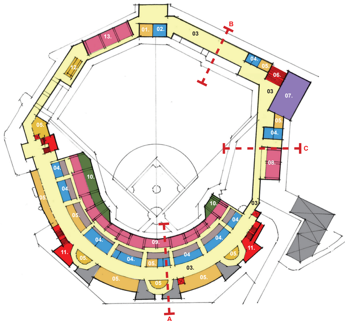
McCoy Stadium - Pawtucket, RI : Renovation Concept - Main Concourse Plan
