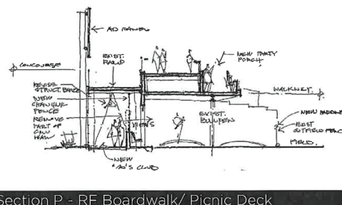
Fig. 012. Populous 2015 Report - Proposed Redevelopment Section
