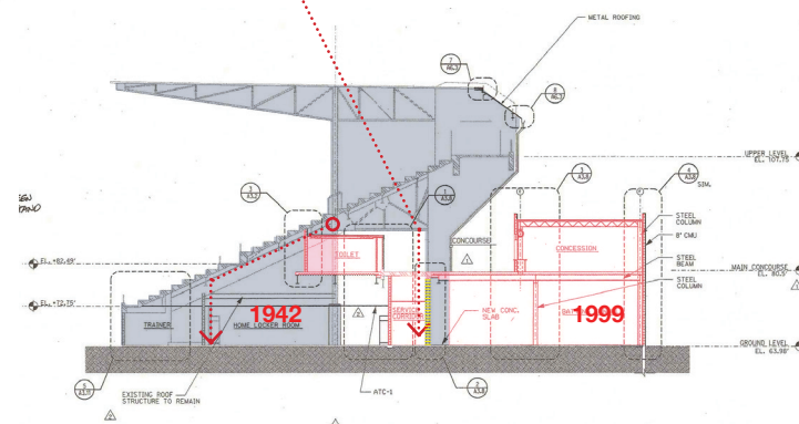
1 BUILDING SECTION @ SADDLEBAG
