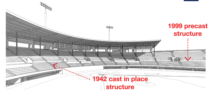
Fig. 098. McCoy Bowl 3D View
